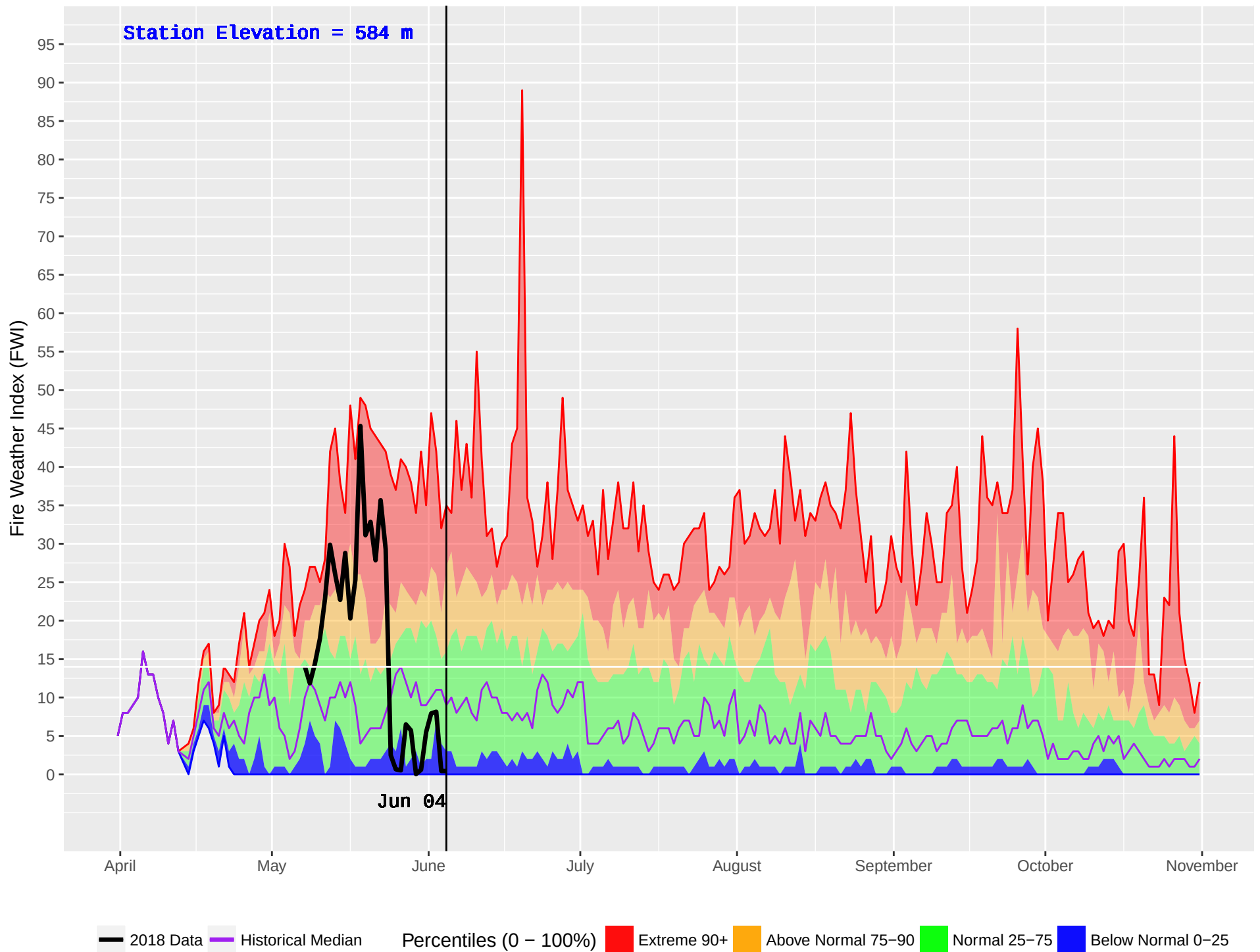
SIERRA (117) : Historical (1981–2016) and Current (2018) Noon Fire Weather Index (FWI)
