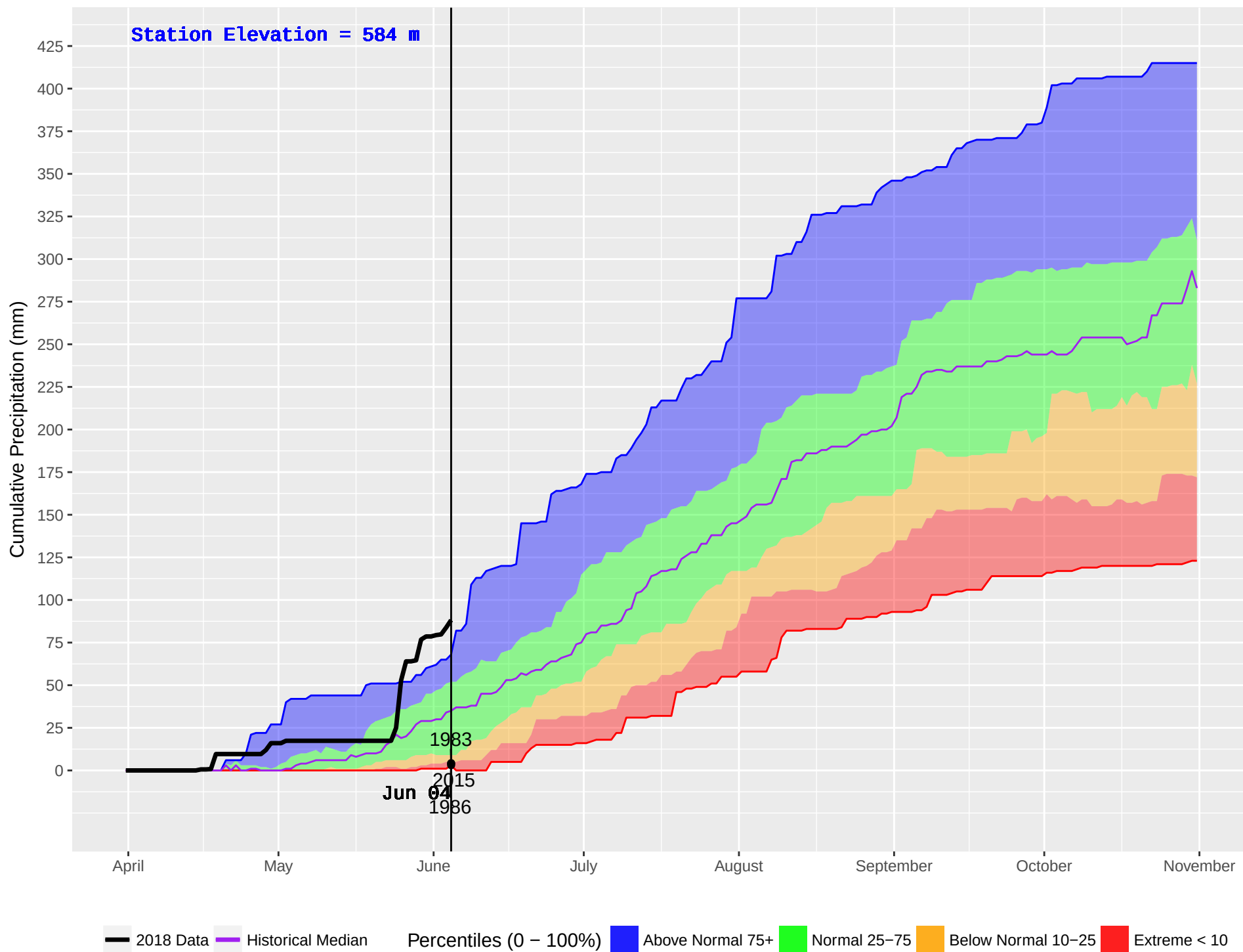
SIERRA (117) : Historical (1981–2016) and Current (2018) Noon Cumulative Precipitation
