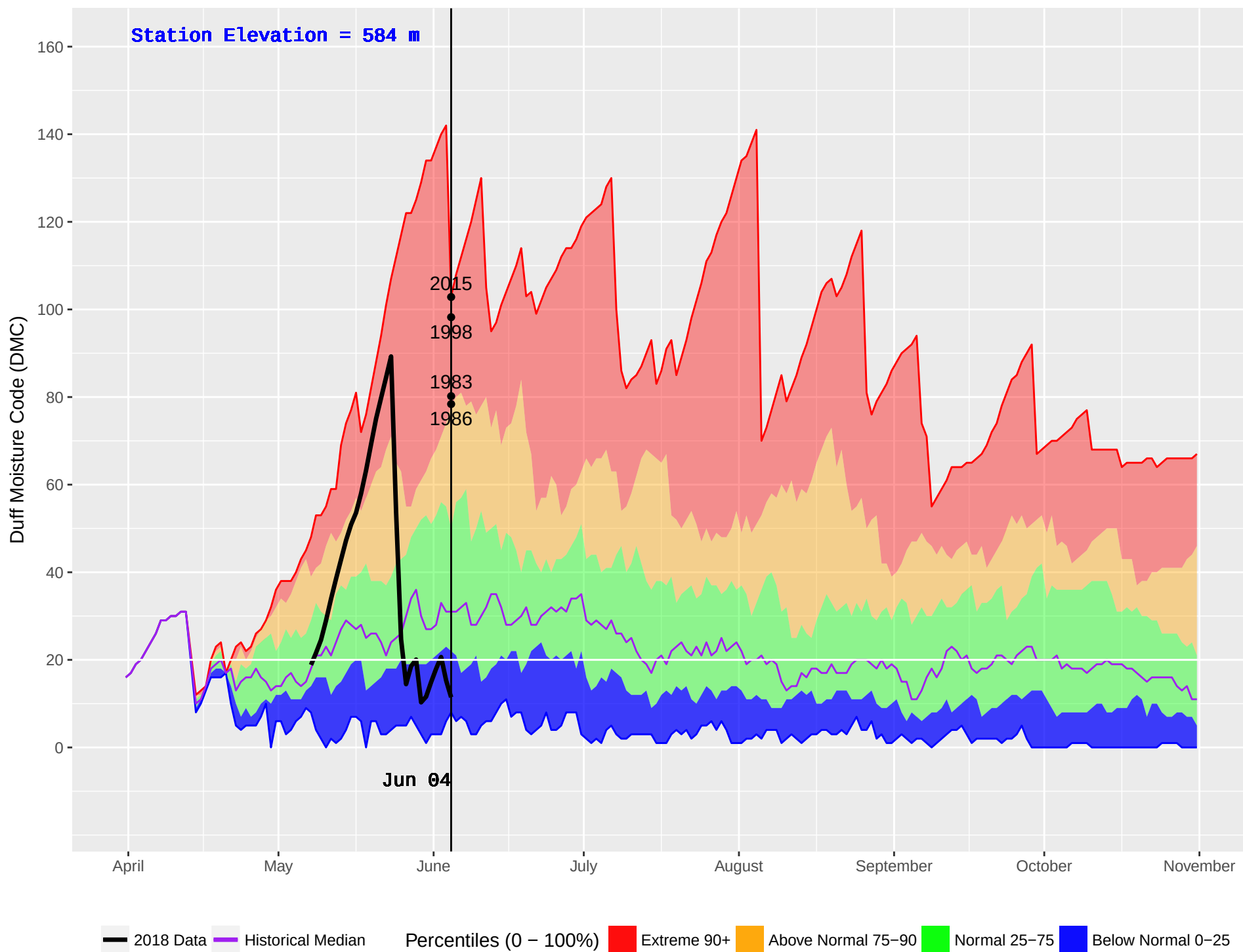
SIERRA (117) : Historical (1981–2016) and Current (2018) Noon Duff Moisture Code (DMC)
